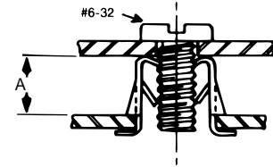
As screw engages legs, sides of part are driven laterally locking part in place.
