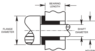
MODEL B Flanged Bearing
