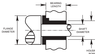
MODEL A Flanged Bearing with Lock Notch
